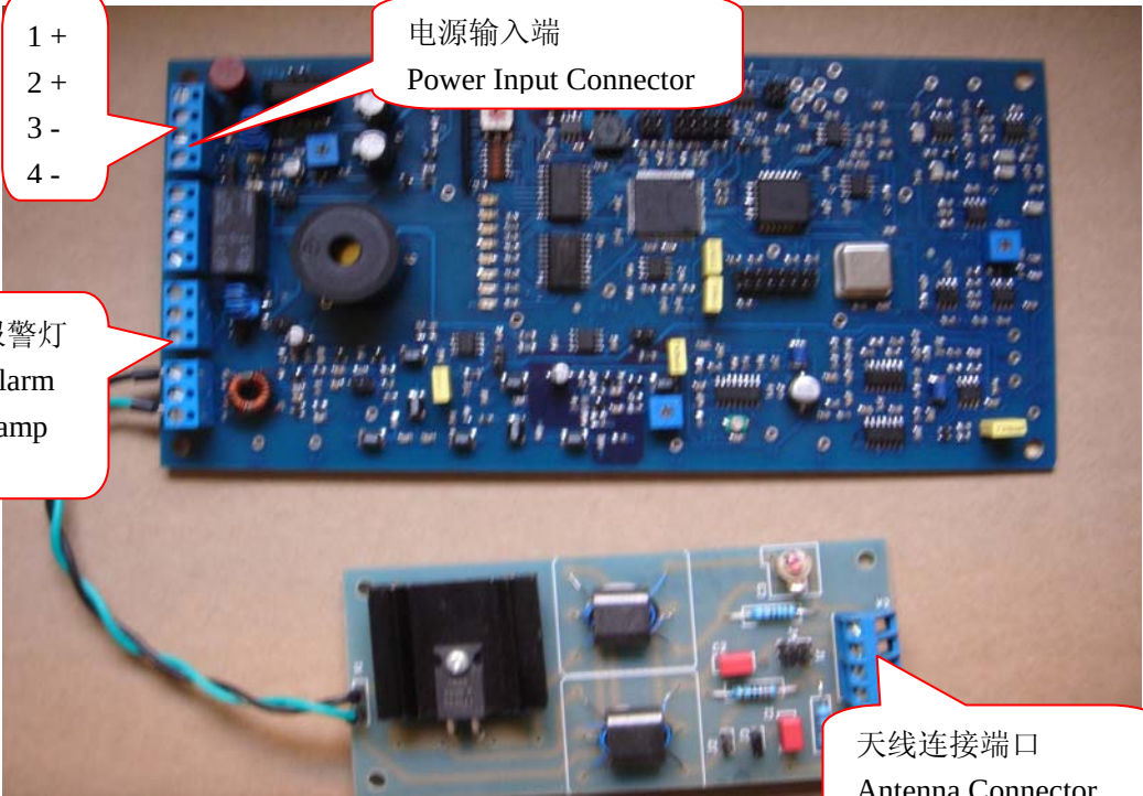
Receive Board 接收板
