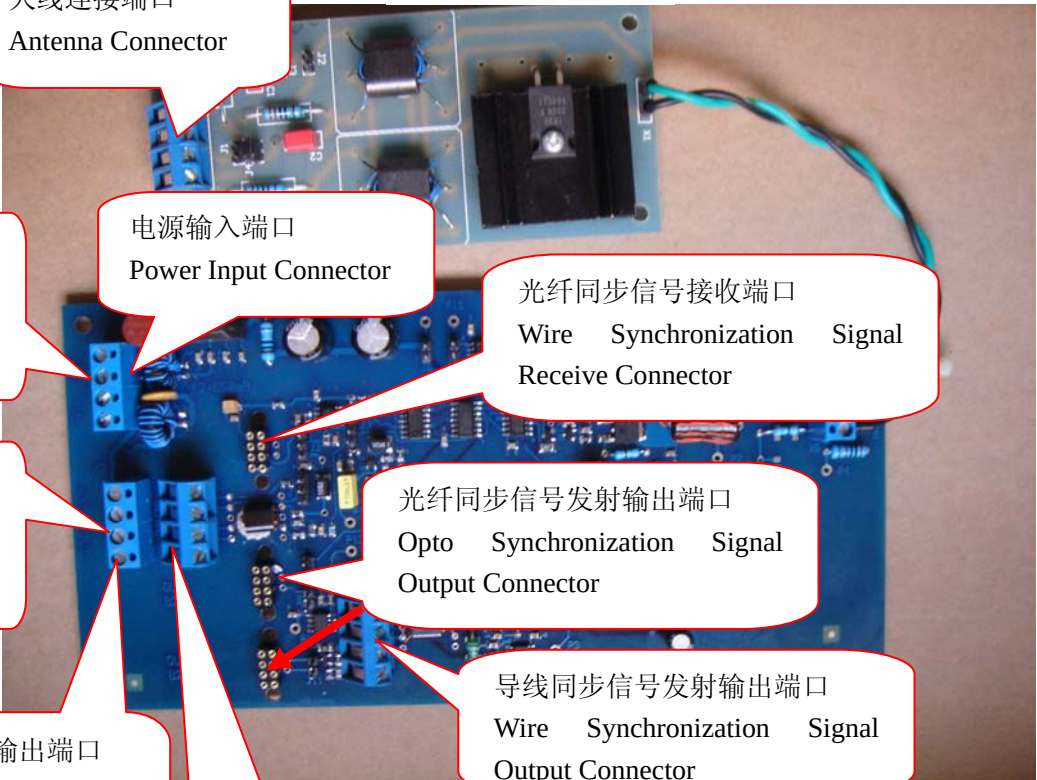
Transmission Board 发射板
